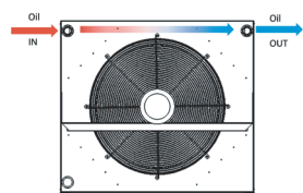
AORF - One Pass with Bypass
