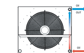
AOFR - Two Pass with Bypass
