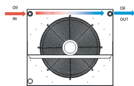
AOFR - One Pass with Bypass
